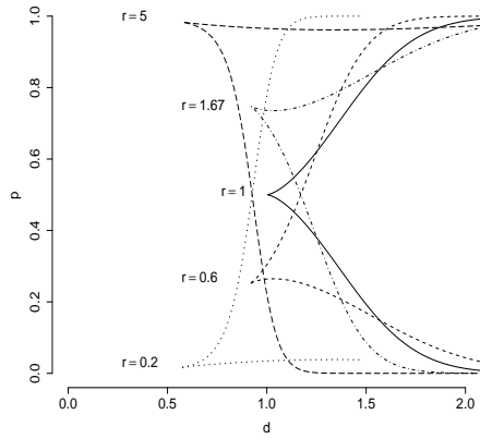
Figure 1: Regions of bimodality of the normal distribution, where d = (\mu_2 - \mu_1)/(2\sqrt{\sigma_1\sigma_2}) and r = \sigma_1/\sigma_2 . On the right side of the curves are those parameter constellations of p and d for which for fixed r the resulting mixture is bimodal.
