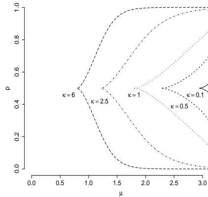
Figure 2: Regions of bimodality of the von Mises distribution, where \mu = \mu_2 - \mu_1 and \kappa_1 = \kappa_2 = \kappa . On the right side of the curves are those parameter constellations of p and \mu for which for fixed \kappa the resulting mixture is bimodal.
